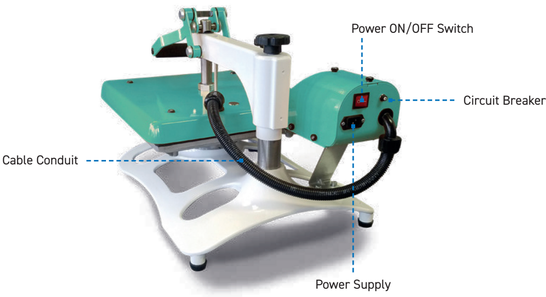
Rear view of heat press
